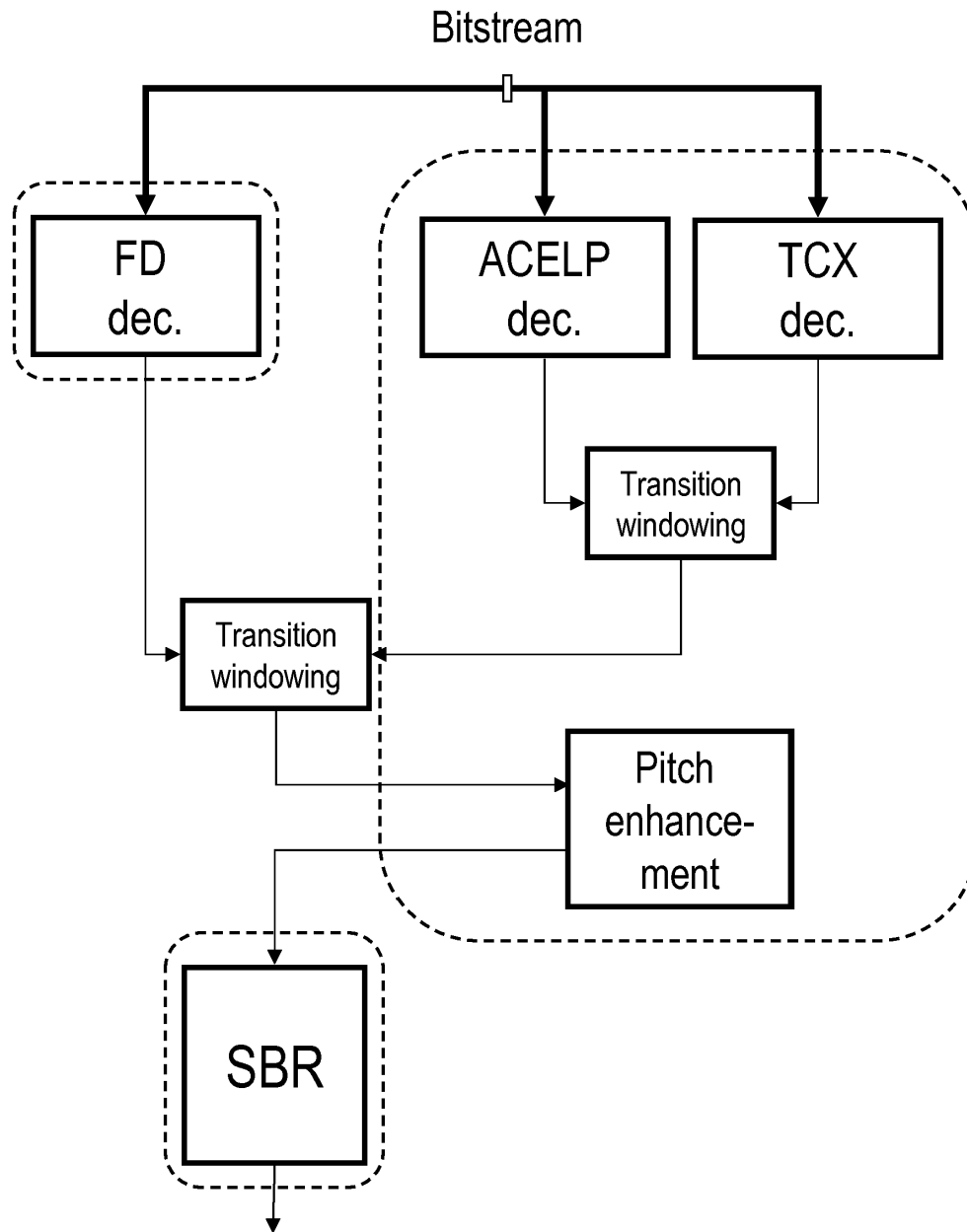
Fig. 6 (prior art)
